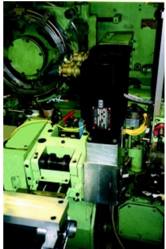
Accu-pac Inner Frame control synchronised drive fitted to GD X2
