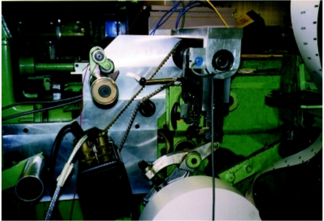
Accu-pac Inner Frame reel unwind fitted to GD X2
